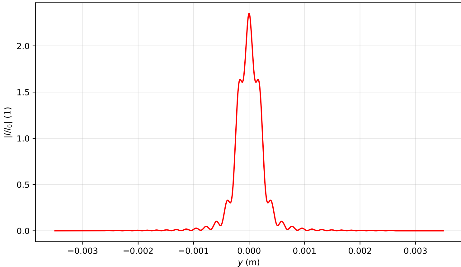
Intensity profile I(x=0, y, z=0.159)/I_0 , P_{in}=1.0P_{cr} , artificial time
